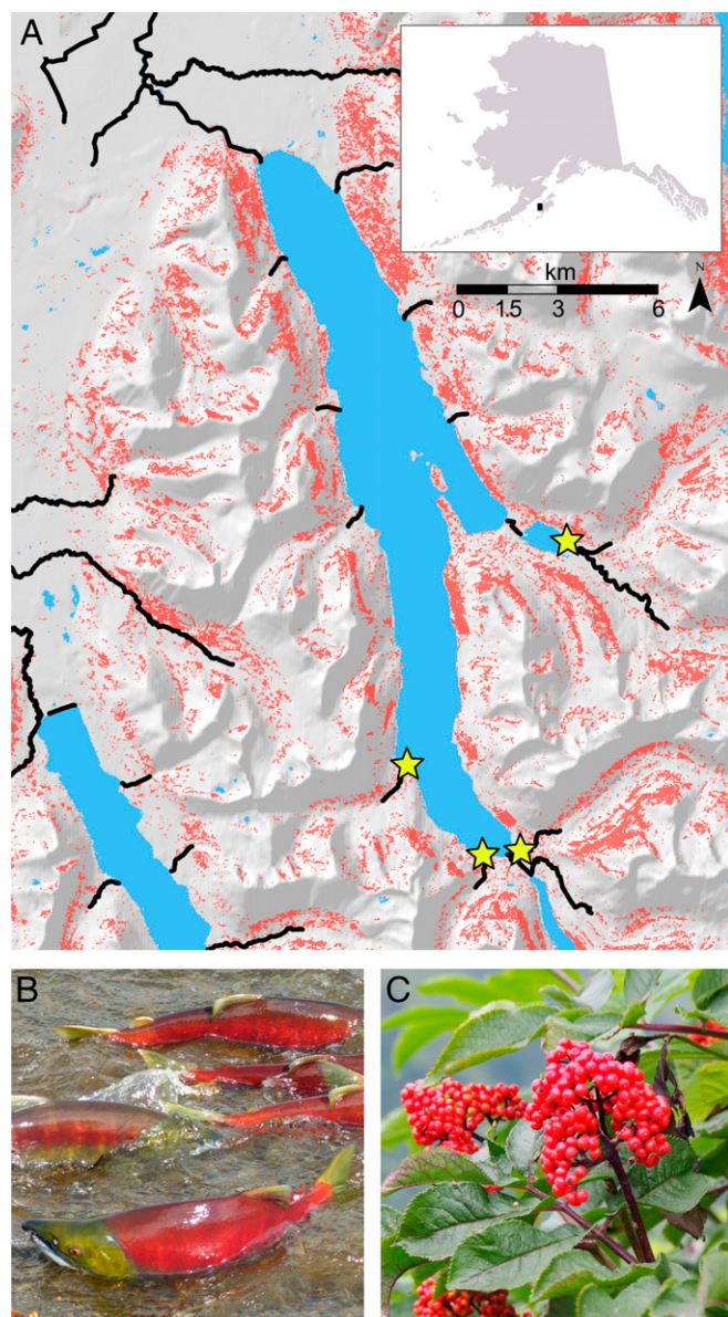
Fig. 1. Key Kodiak brown bear trophic resources and their distribution. (A) Map of the study system showing areas with 10–40% red elderberry land cover (red), and the streams/tributaries where sockeye salmon ( Oncorhynchus nerka ) spawn (black lines). Yellow stars indicate the four focal tributaries where we quantified salmon abundance and monitored bear activity. (B) Spawning sockeye salmon entering a tributary stream within the study area. (C) Red elderberry shrub with ripe berries.
